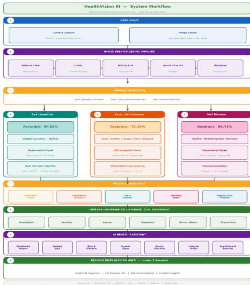
Figure 4.1: HealthVision AI Complete System Workflow Diagram
